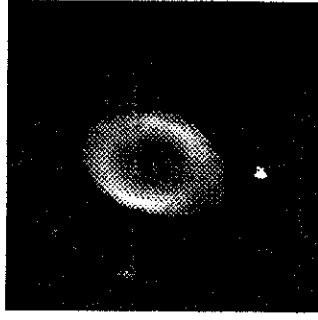
M57 B/W Version of Color CCD Image
