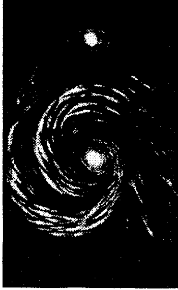
M51. The First Known Spiral Galaxy as it Appeared in the 72" Telescope. This drawing is by Lord Rosse himself.
