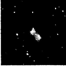
M76 Planetary in Perseus
